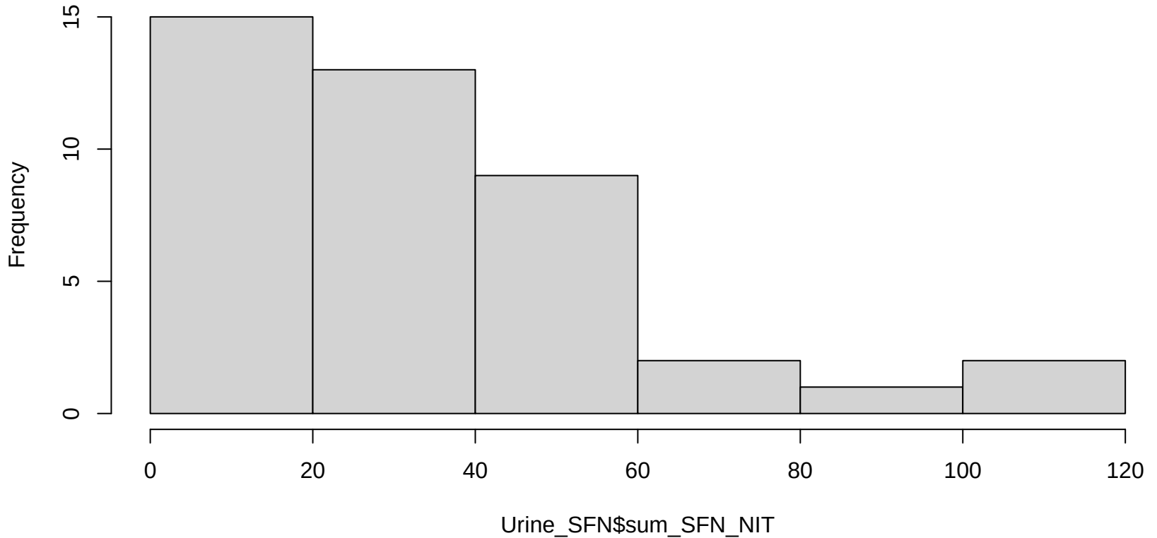
Histogram of Urine_SF_N$sum_SF_N_NIT
